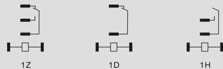
JQX-50F 1Z Wiring diagram (Bottom view)
